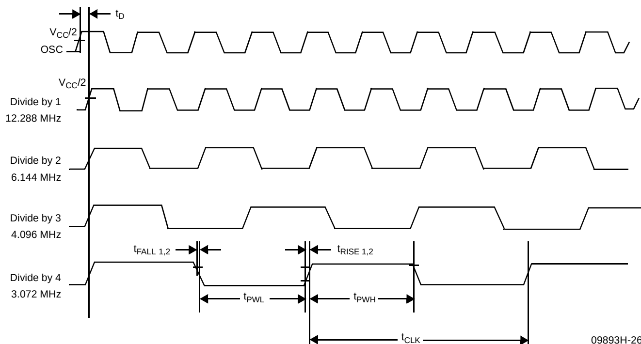
Figure 34. OSC/MCLK Timing
