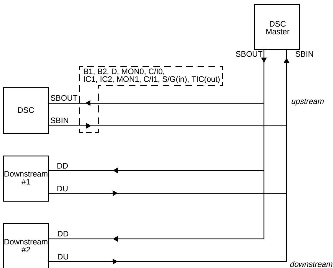
Figure 10. IOM-2 Slave Mode Operation without Bus Reversal
