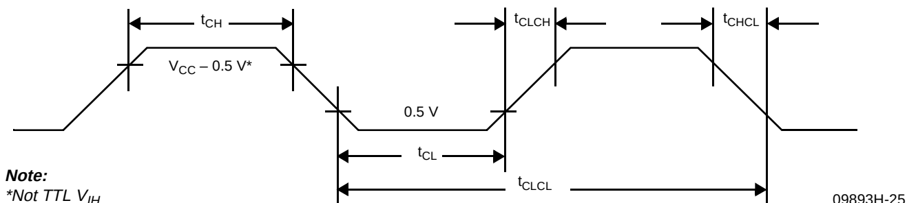
Figure 33. External Clock Driver (XTAL2) Timing
