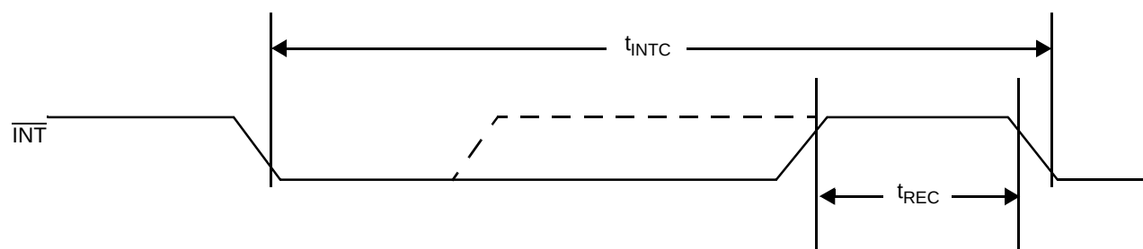
Figure 30. \overline{INT} Timing
