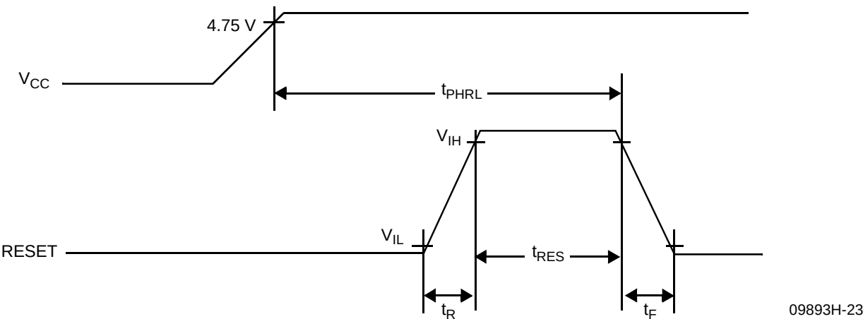
Figure 31. Reset Timing
