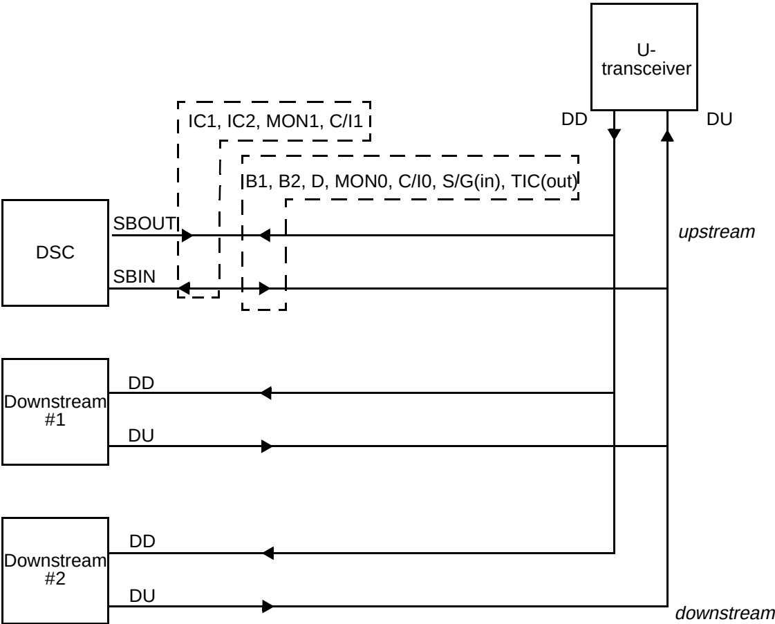
Figure 9. IOM-2 Slave Mode Operation with Bus Reversal
