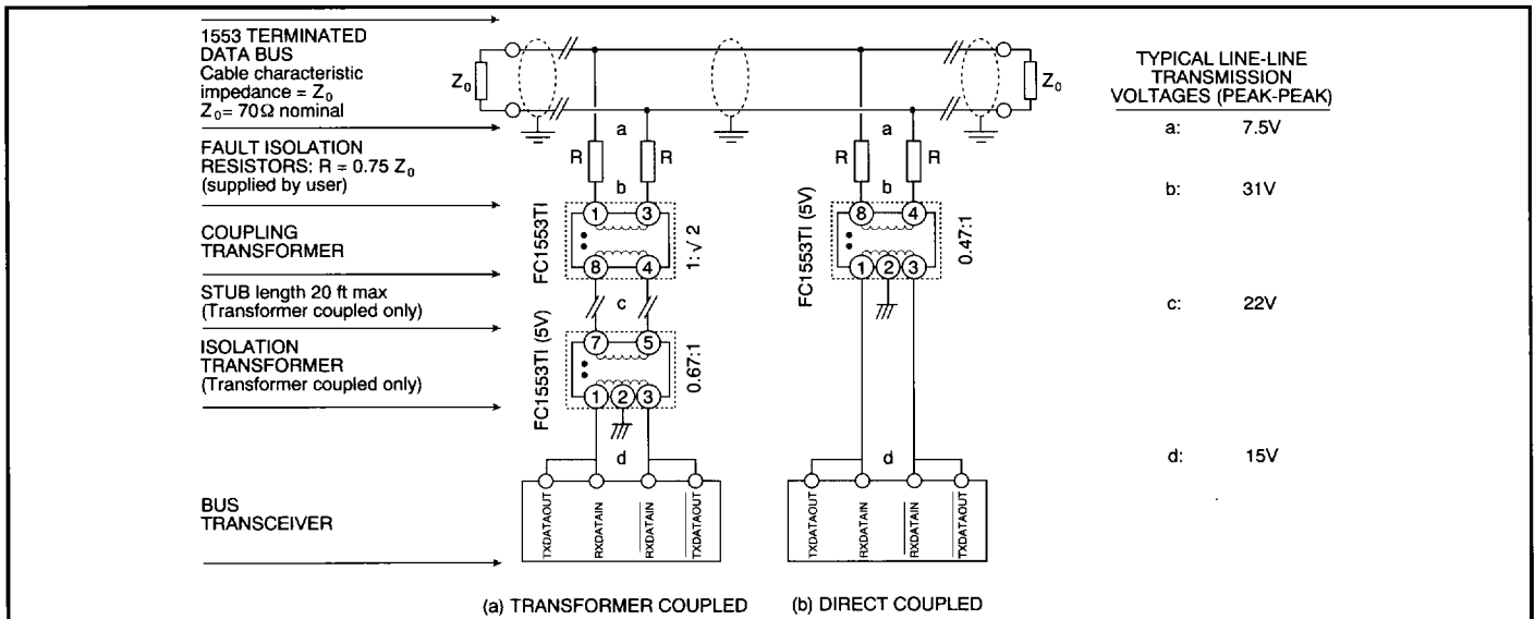
Fig. 4 Transceiver to bus connection diagram
