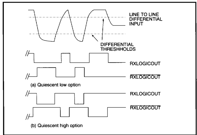
Fig. 6 Typical receiver waveforms
