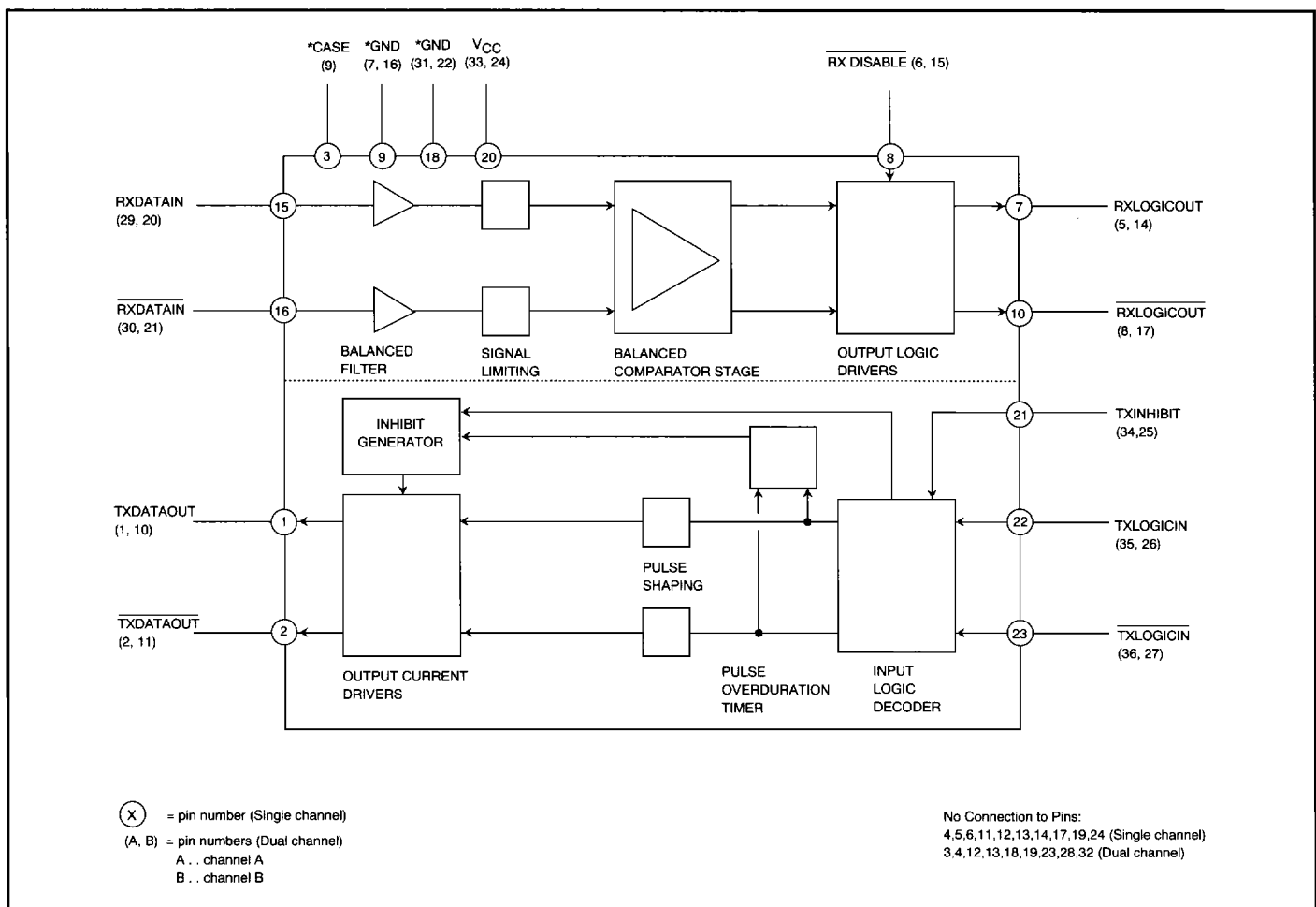
Fig. 1 Block Schematic
