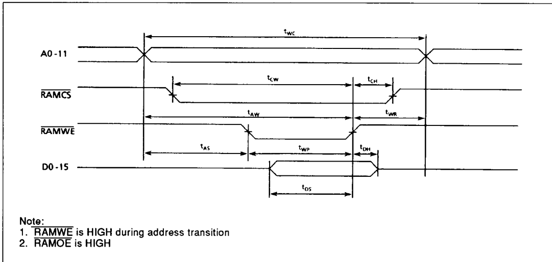
Figure 17: Timing Waveform of Write Cycle
