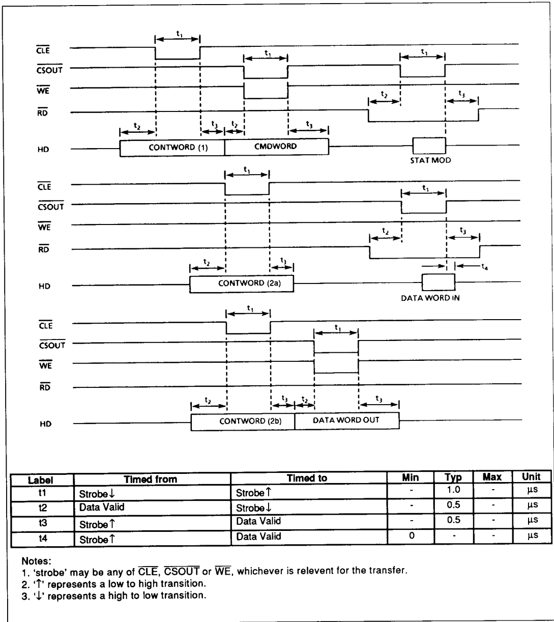
Figure 26: STANAG 3910 Interface Timing Details (refer to Figures 25a and 25b for basic transfers)
