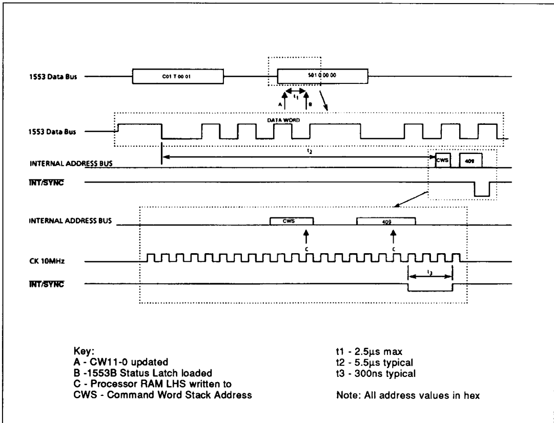
Figure 9: Synchronise without Data Word Mode Command
