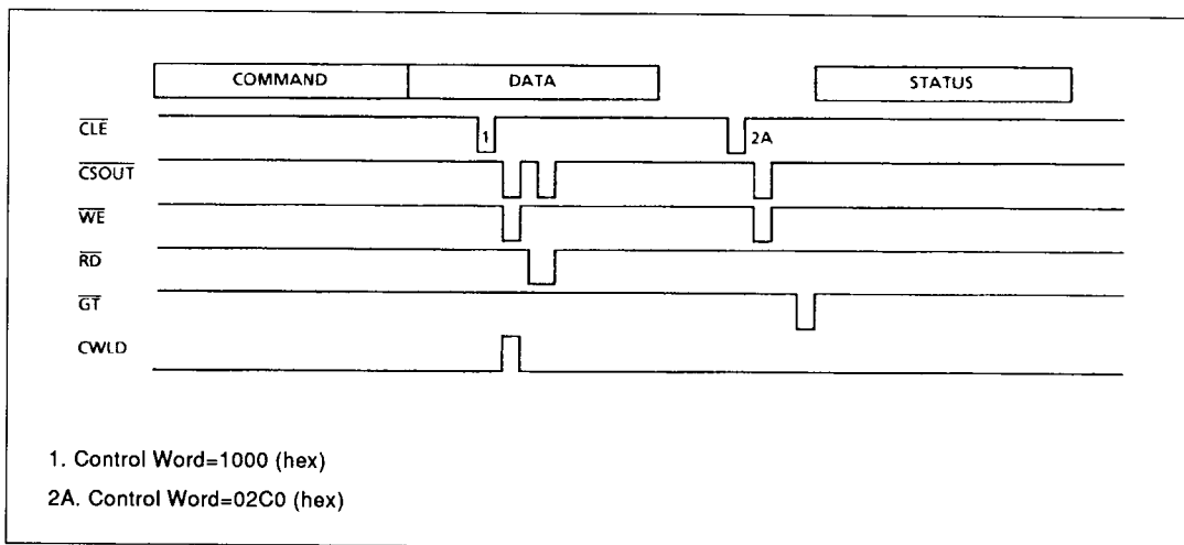
Figure 25a: Receive Command - 1 Word Subaddress 22
