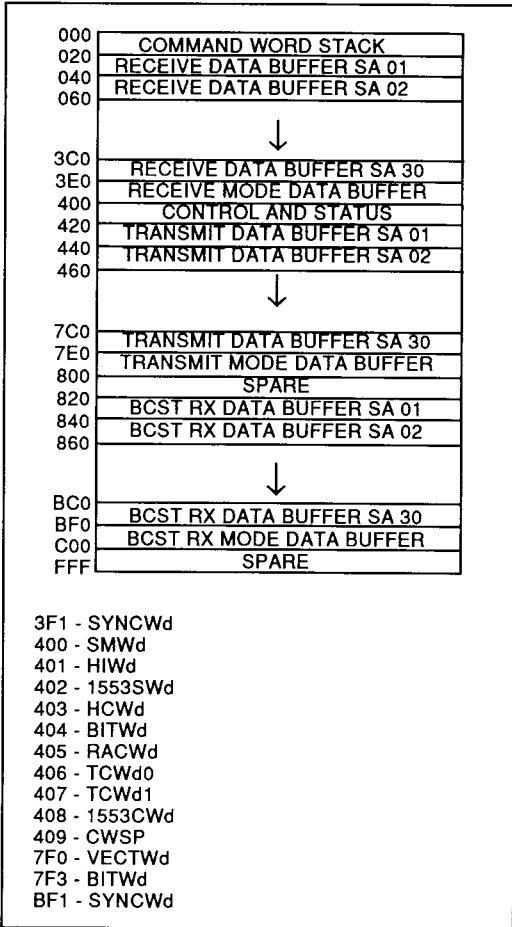
Figure 5: Memory Architecture
