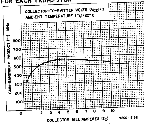
Fig.15 - Typical gain-bandwidth product vs collector current.
