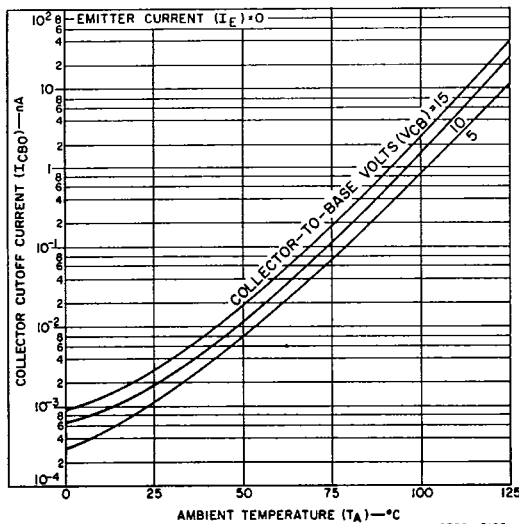
Fig.2 - Typical collector-to-base cutoff current vs ambient temperature for each trans
