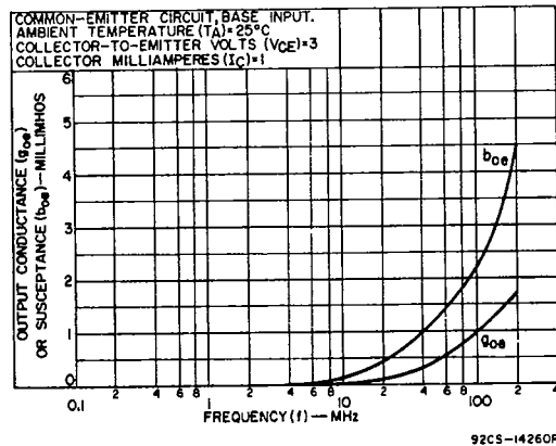
Fig.13 - Typical output admittance vs frequency.
