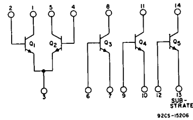
Fig.1 - Schematic diagram.
