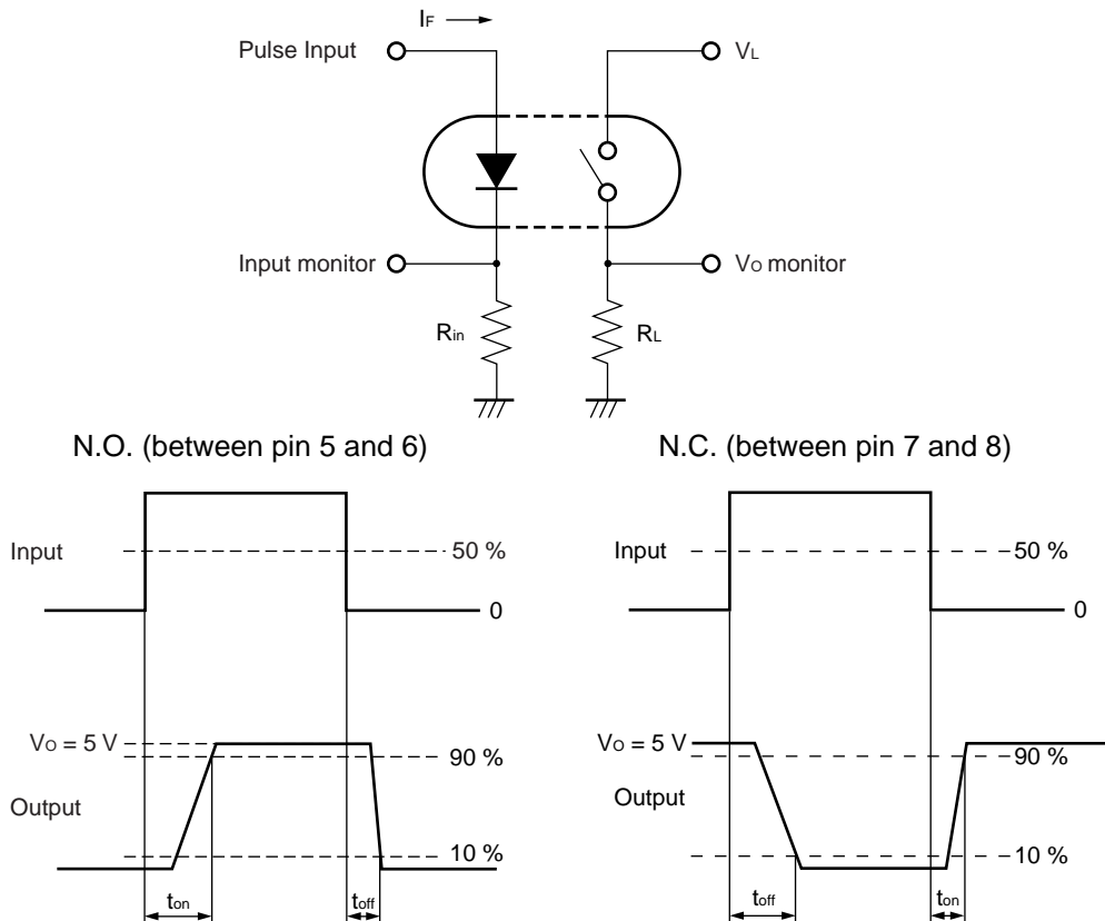
*1 Test Circuit for Switching Time
