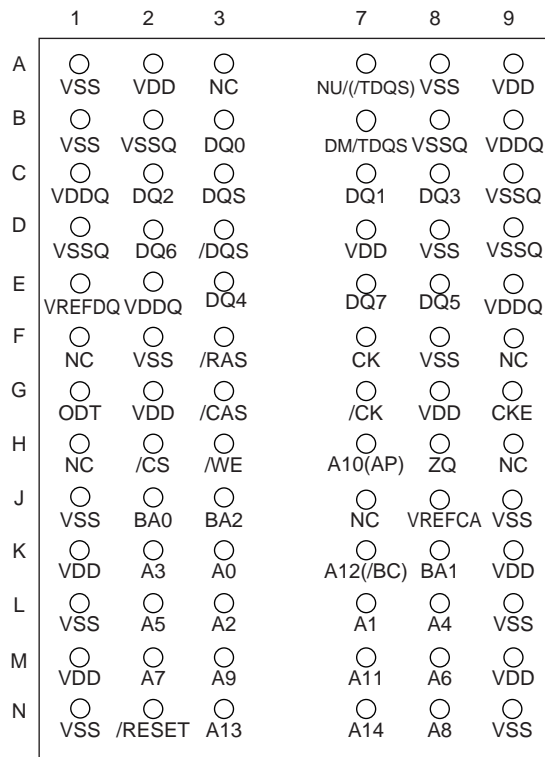
(Top view)
