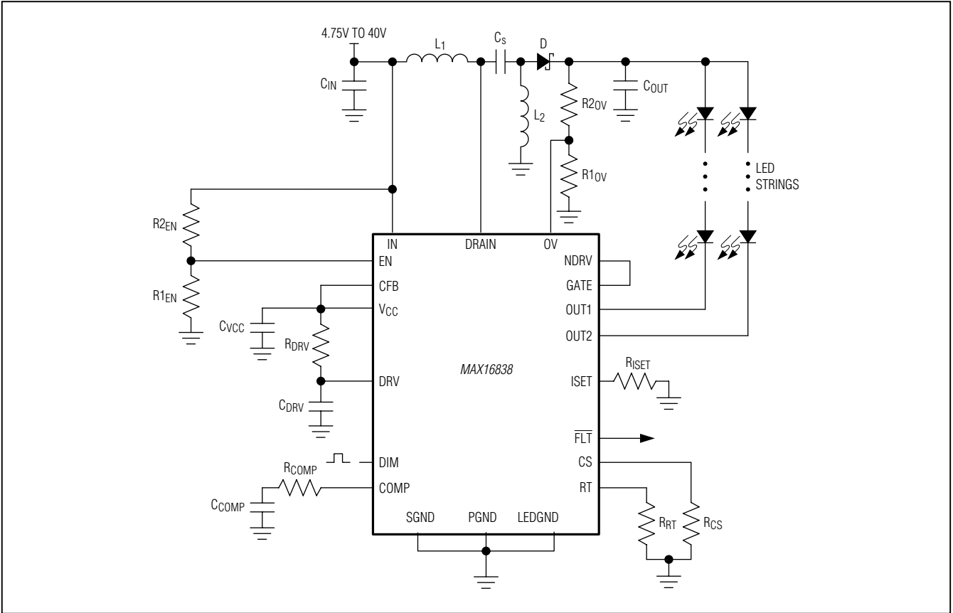
Figure 4. SEPIC Configuration
