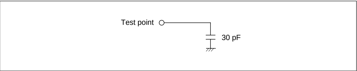
Figure 9 Load Circuit
