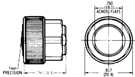
7mm Precision Connector (Hermaphrodite)
