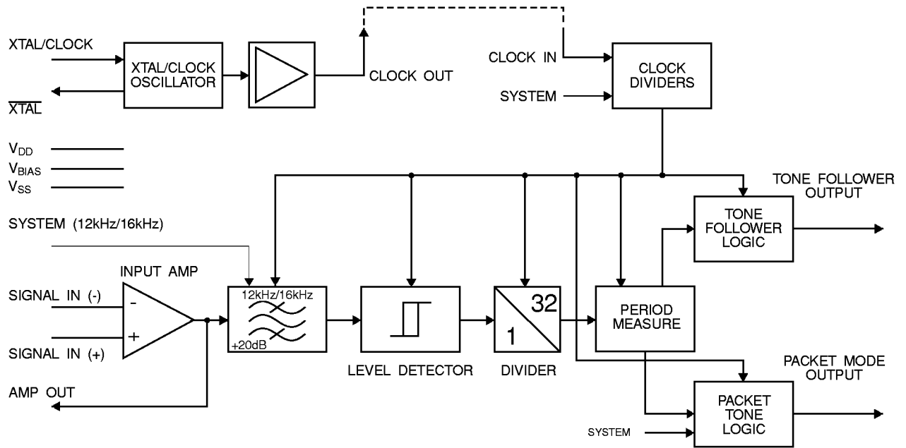
Figure 1: Block Diagram
