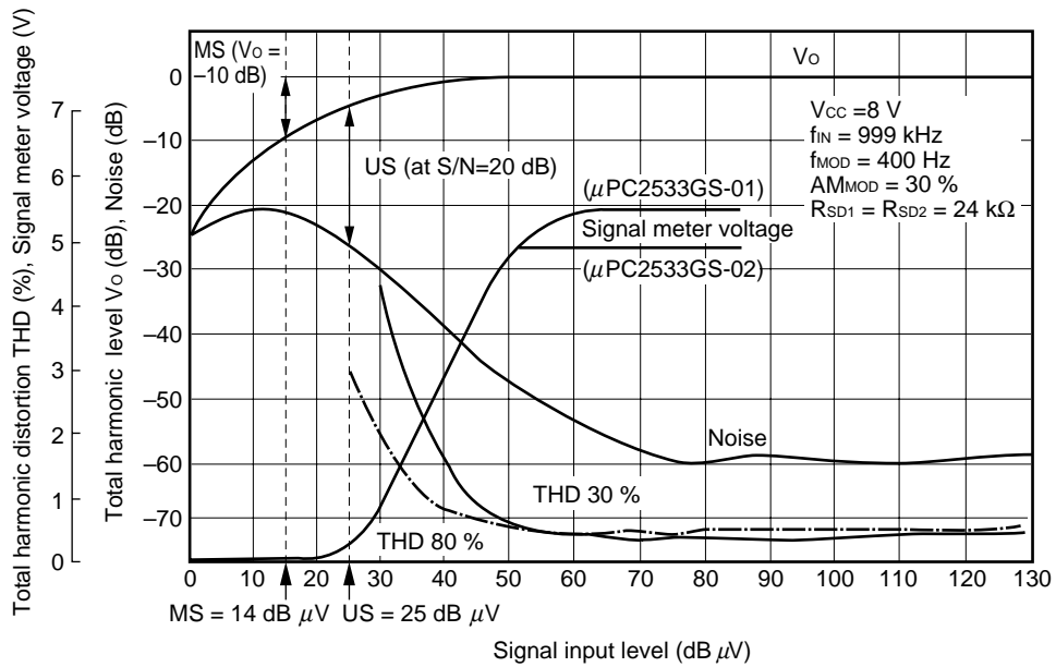
Input/Output Characteristics (1)
