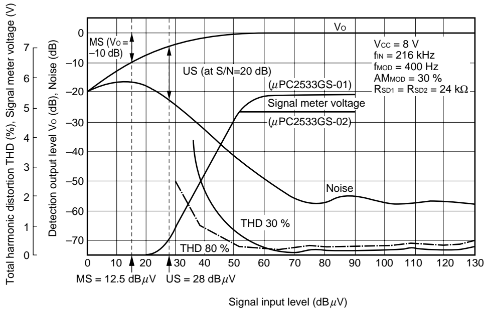
Input/Output Characteristics (2)
