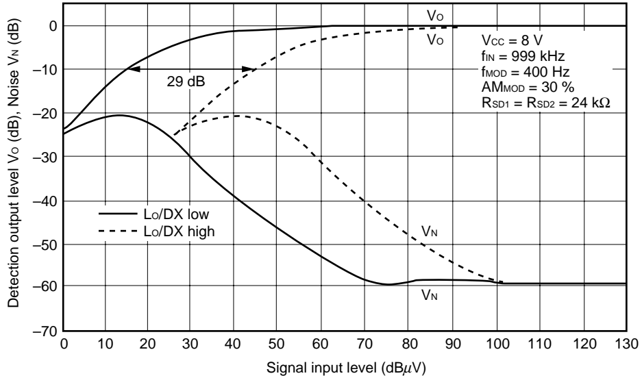
Input/Output Characteristics (4)
