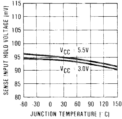
Sense Input Hold Voltage vs Junction Temperature
