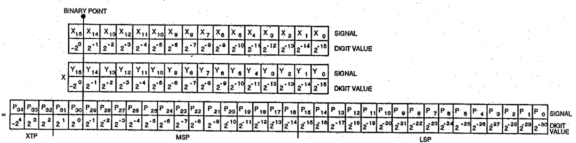
Figure 6. Fractional Two's Complement Notation
