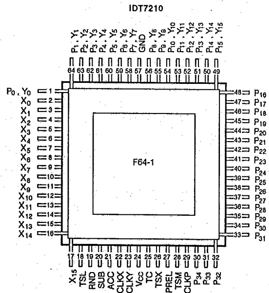
FLATPACK TOP VIEW
