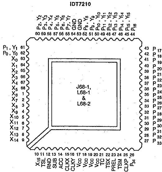
LCC/PLCC/FINE-PITCH LCC TOP VIEW
