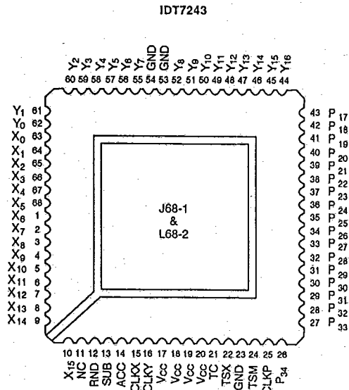
LCC/PLCC TOP VIEW
