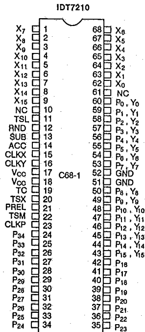
SHRINK-DIP TOP VIEW
