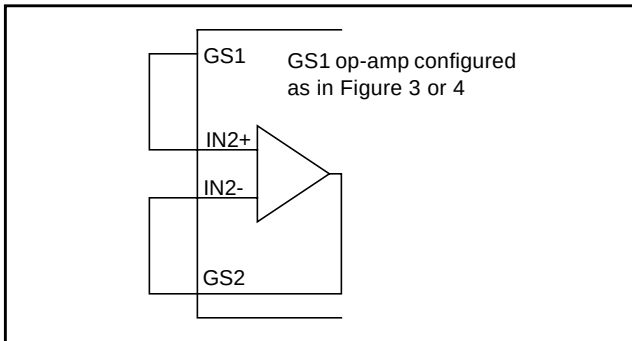
Figure 5 - GS2 Op-Amp Connected as GS1 Voltage Follower
