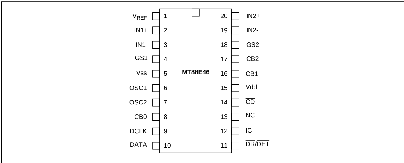
Figure 2 - Pin Connections
