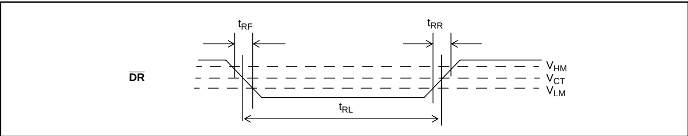
Figure 11 - \overline{DR} Output Timing
