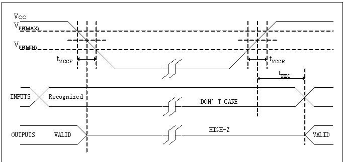
Fig 3. Power-Up/Power-Down Timing
