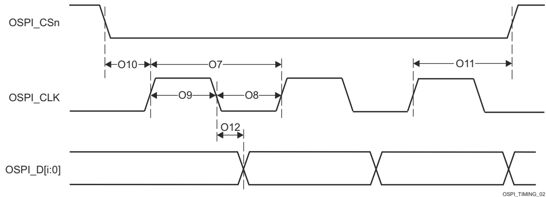
Figure 7-103. OSPI0 Switching Characteristics – Tap SDR, No Loopback
