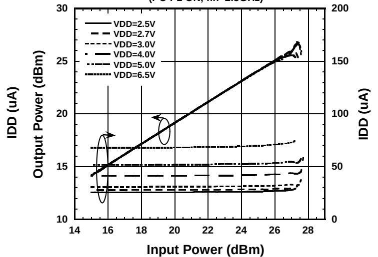
Output Power, IDD vs. Input Power
