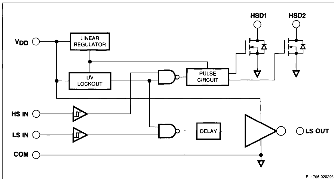
Figure 3. Functional Block Diagram of the INT202
