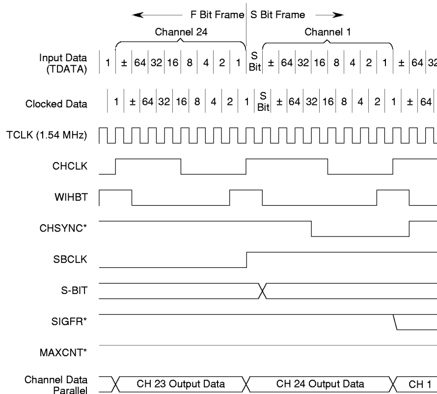
Figure 2. Signal Relationships at Beginning of F_S Frame (S-BIT).
