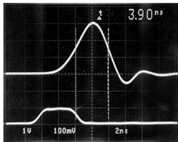
Minimum Output Pulse Width
