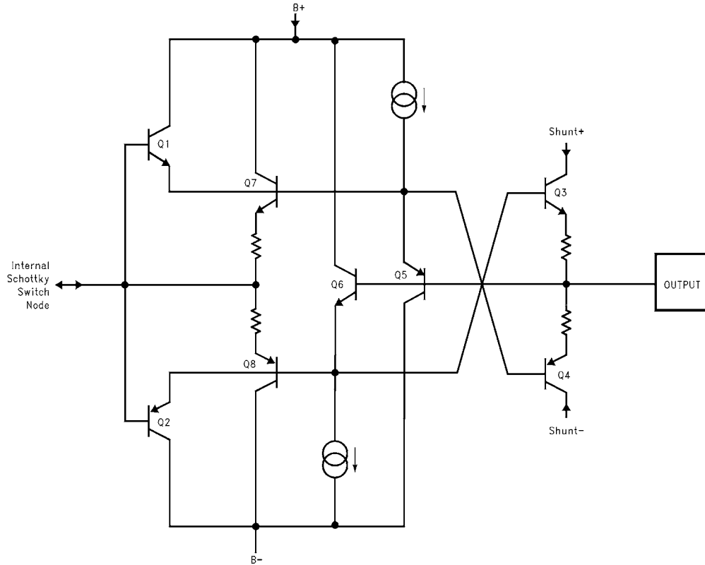
FIGURE 3. OUTPUT STAGE CIRCUIT IN THREE-STATE MODE
