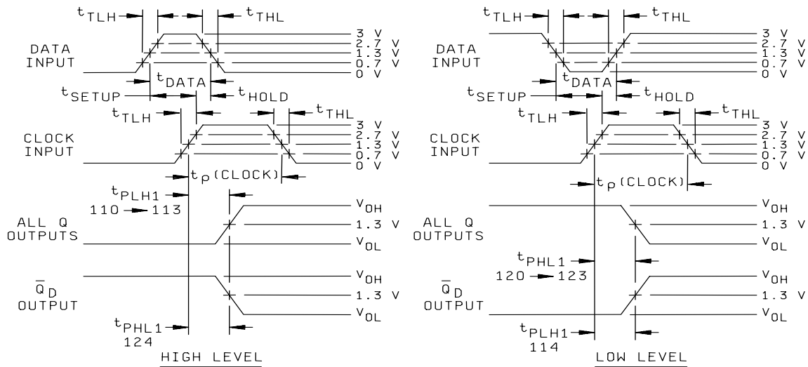
CLOCK TO OUTPUT WAVEFORMS (PARALLEL INPUT)
