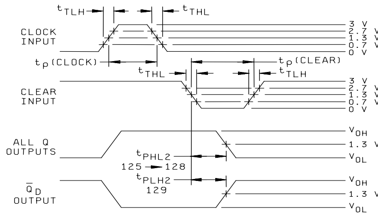
CLEAR TO OUTPUT WAVEFORMS
