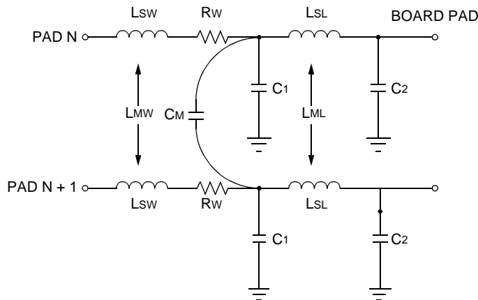
Figure 66. Package Parasitics
