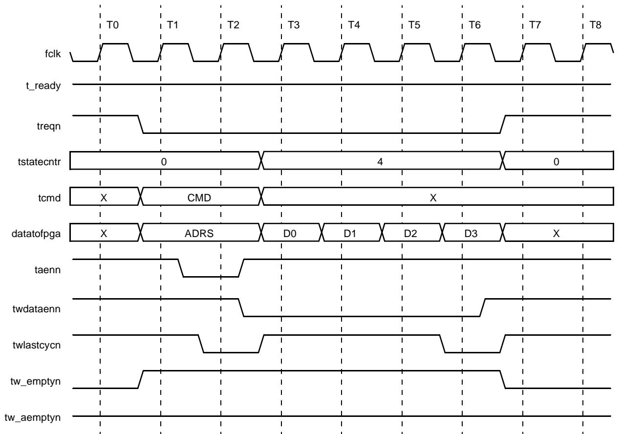
Figure 15. Target Write Memory 32-Byte Burst (FPGA Bus, Dual-Port)
