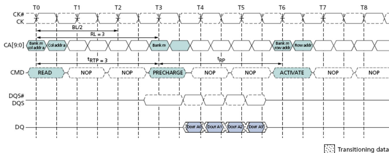
Burst Read followed by Precharge: RL=3, BL=4, RU( \frac{t_{RTP}(\text{min})}{t_{CK}} ) = 3
