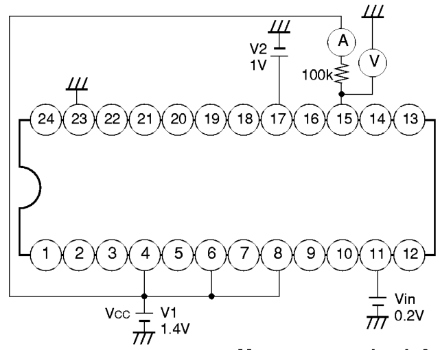
Measurement circuit 8
