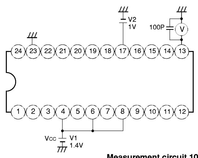
Measurement circuit 10
