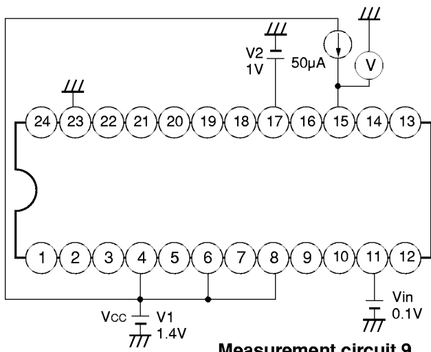
Measurement circuit 9
