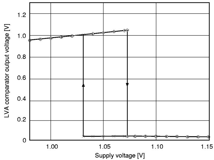
LVA characteristics
