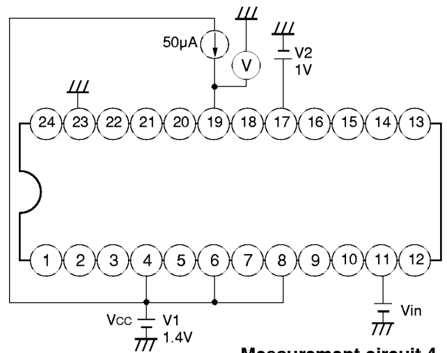
Measurement circuit 4
