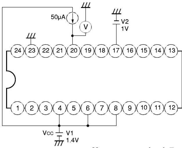
Measurement circuit 7
