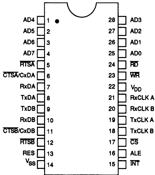
28-Pin DIP
