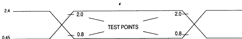
Figure 9. Test Points
