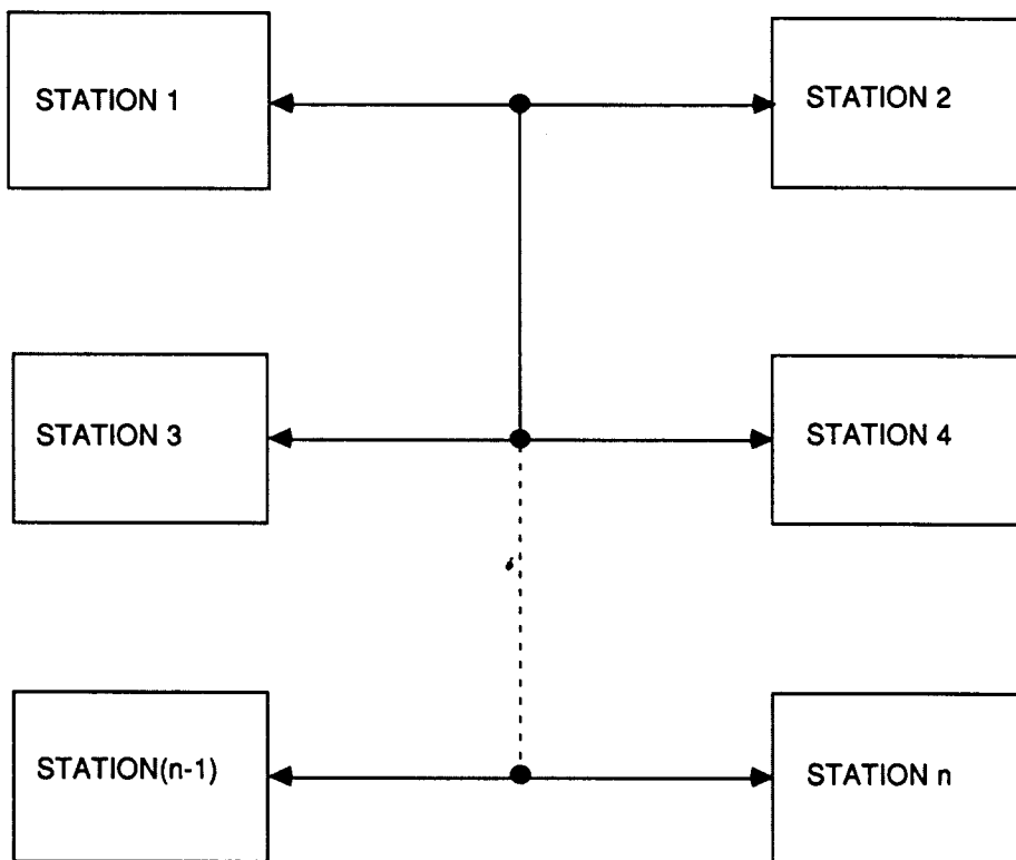
Figure 3. Multimaster Configuration
