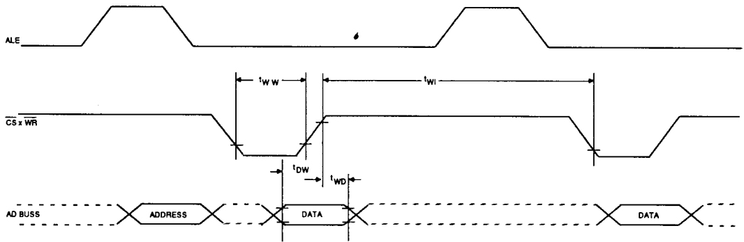
Figure 5. Write Cycle
