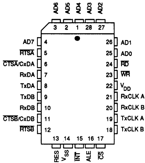
28-Pin PLCC
