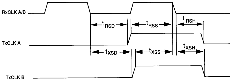
Figure 8. Clock Mode 1
