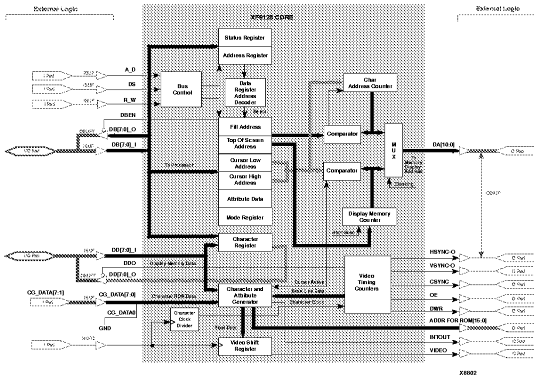
Figure 1: XF9128 Video Terminal Logic Controller Block Diagram
