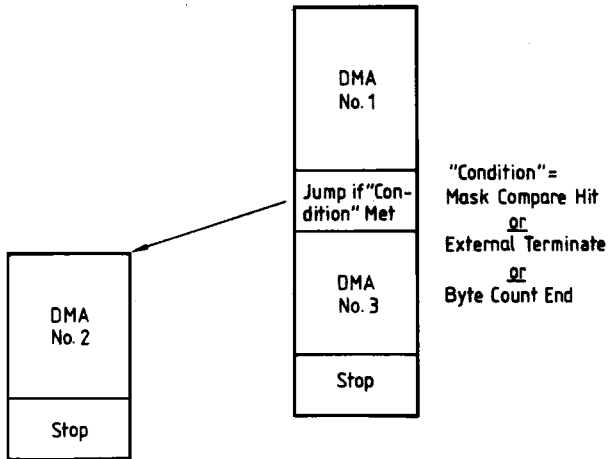
c) Conditional DMA Operation
