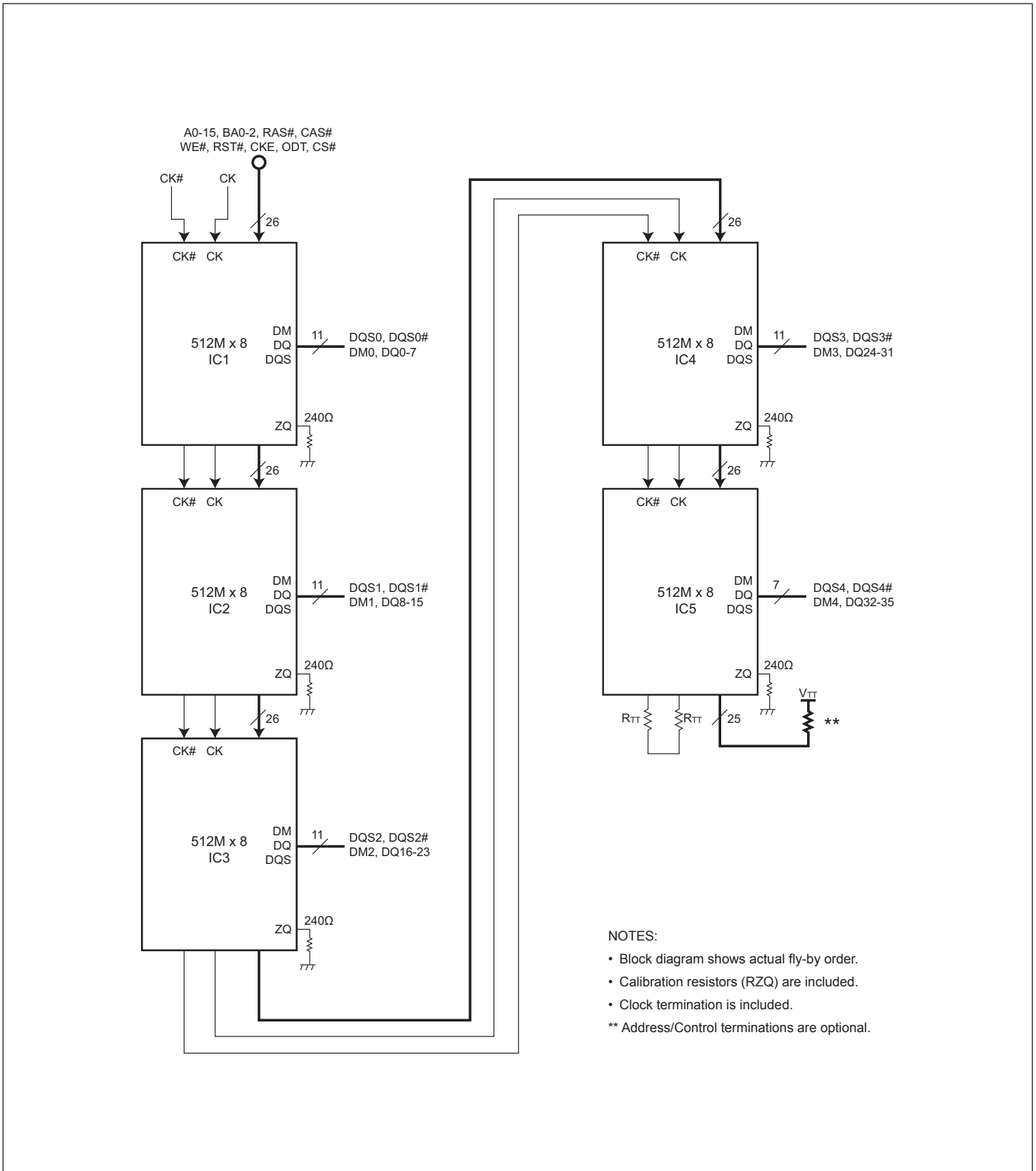
FIGURE 2C – FUNCTIONAL BLOCK DIAGRAM FOR W3J512M36K(T)-XB3X
