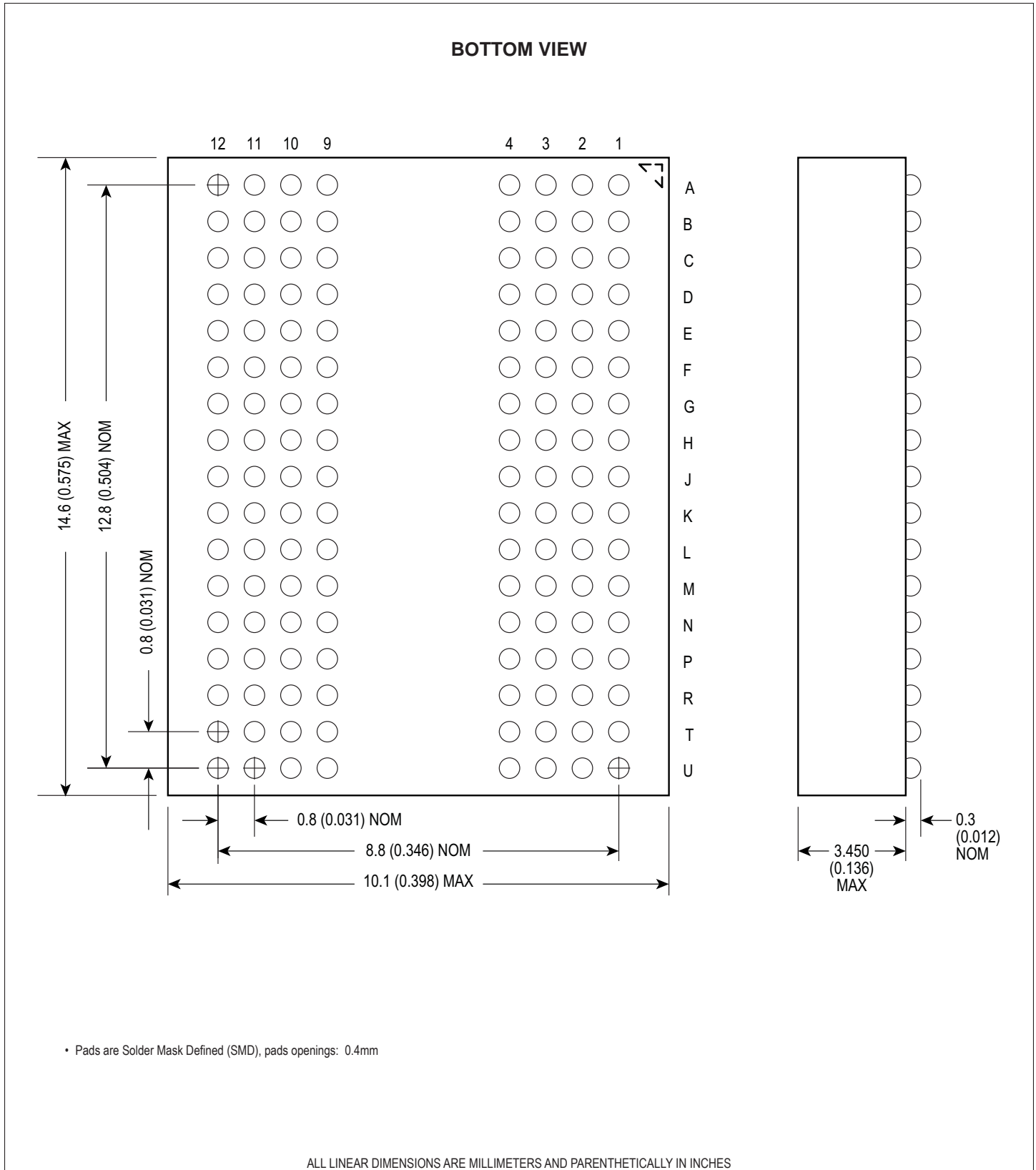
FIGURE 16 – PACKAGE DIMENSION: 136 PLASTIC BALL GRID ARRAY (PBGA) for W3J512M32K-XBX
