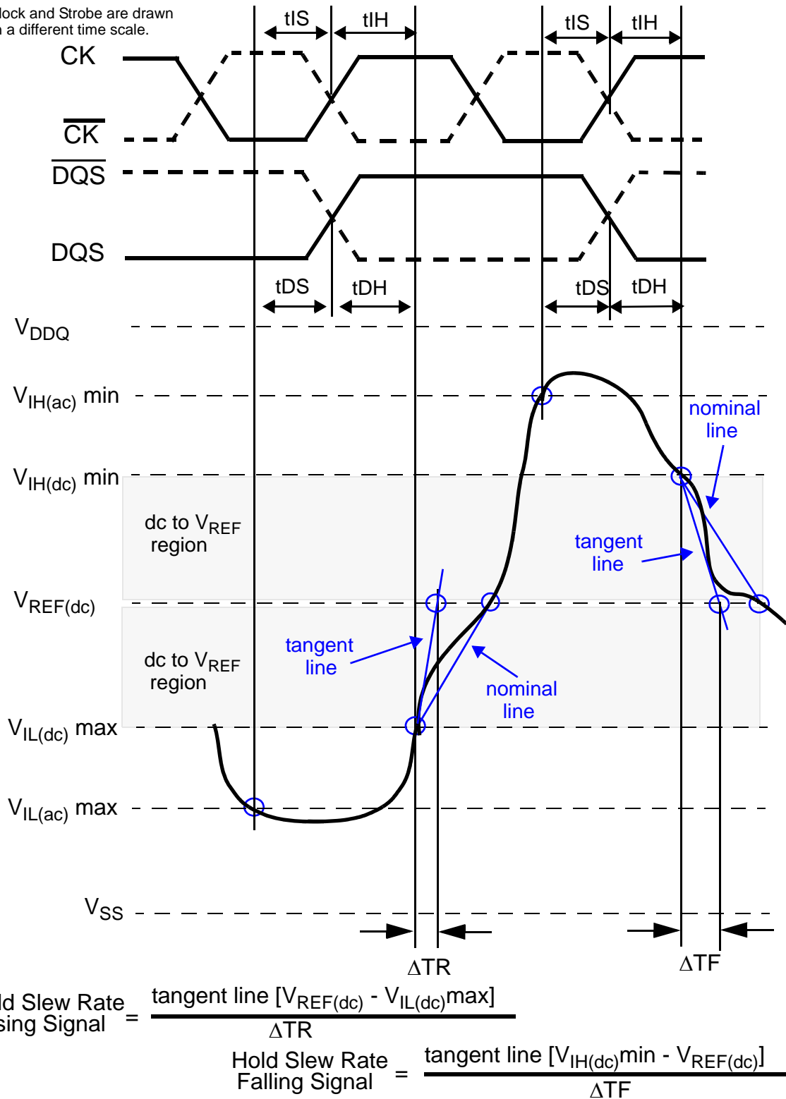
Figure 10 - Illustration of tangent line for hold time t_{DH} (for DQ with respect to strobe) and t_{IH} (for ADD/CMD with respect to clock).
