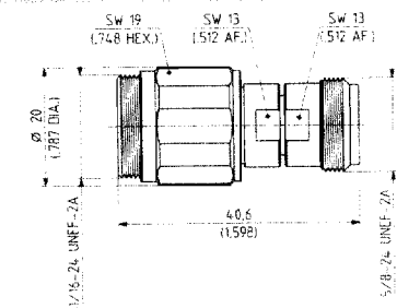
TYPE 33 PC7-N-50-1
