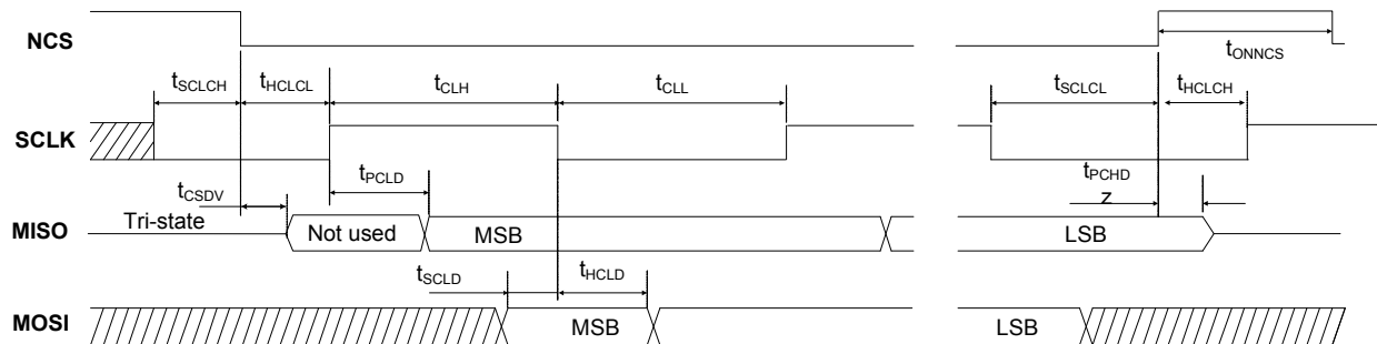
Figure 7. SPI Timing Diagram
