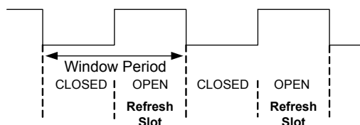
Figure 16. Windowed Watchdog
