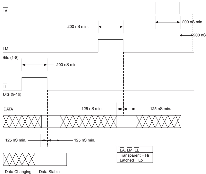
FIGURE 2B. LL, LM, LA TIMING DIAGRAMS (8 BIT)
