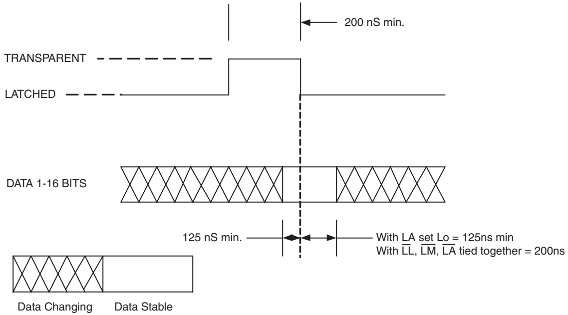
FIGURE 2A. LL, LM, LA TIMING DIAGRAMS (16 BIT)
