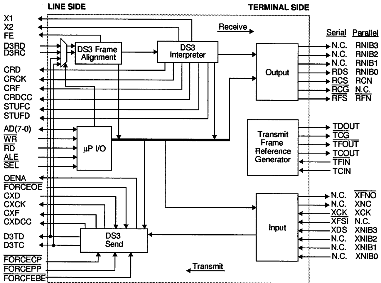
Figure 1. DS3F TXC-03401 Block Diagram
