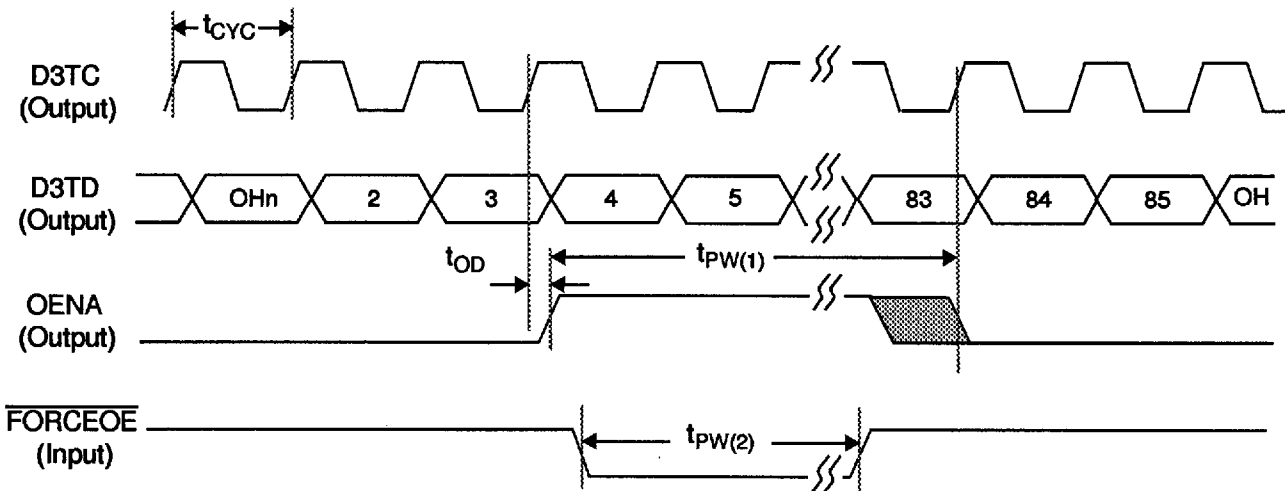
Figure 13. Force Overhead Bit Error Timing (FORCEOE)
