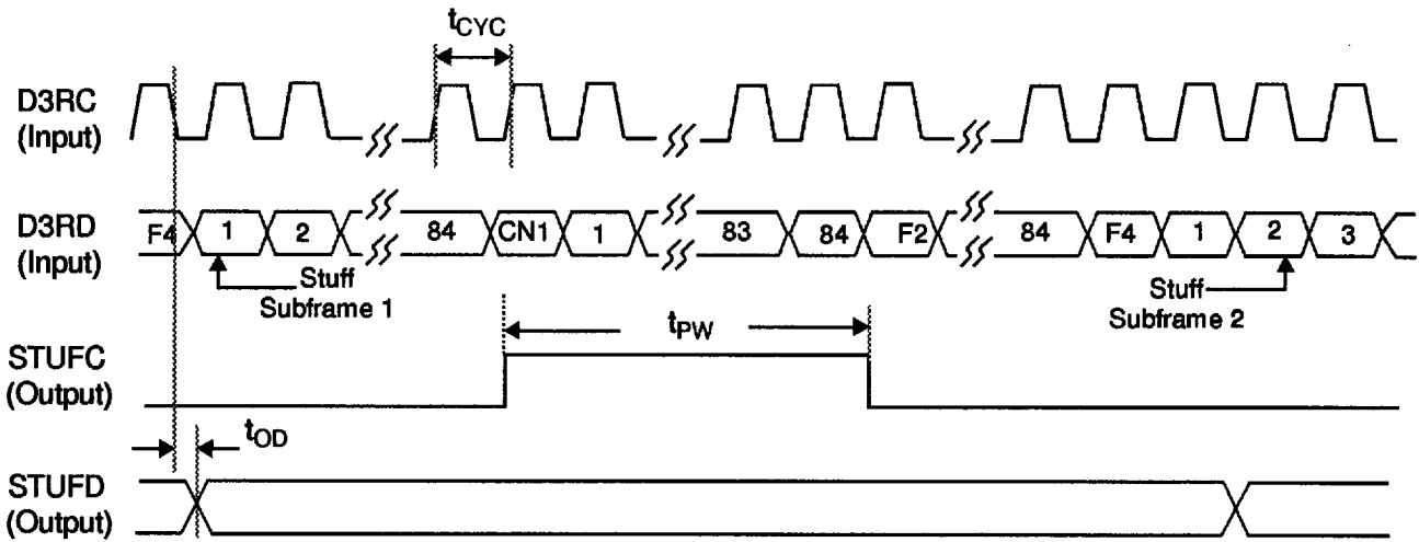
Figure 14. Stuff Opportunity Bit Timing (M13 Mode)
