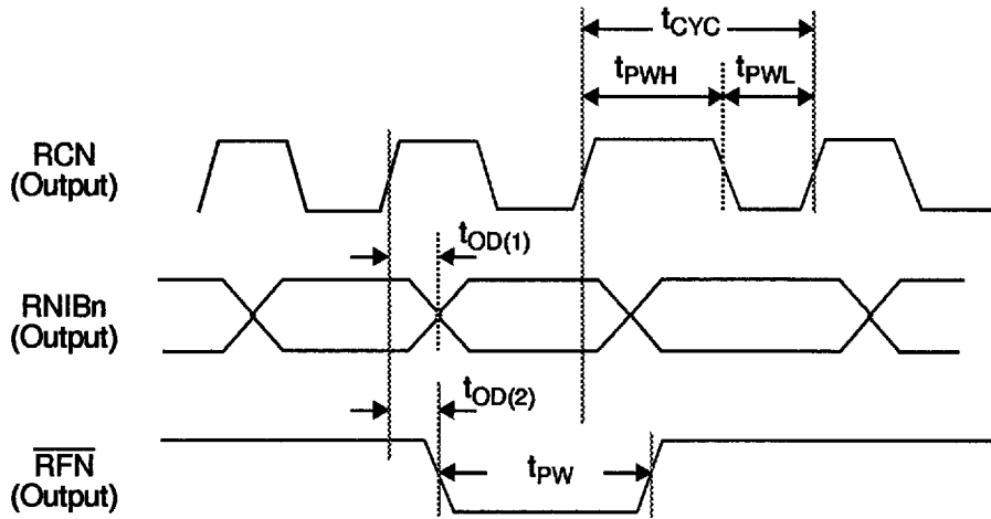
Figure 5. Terminal Side Receive Nibble Output Timing
