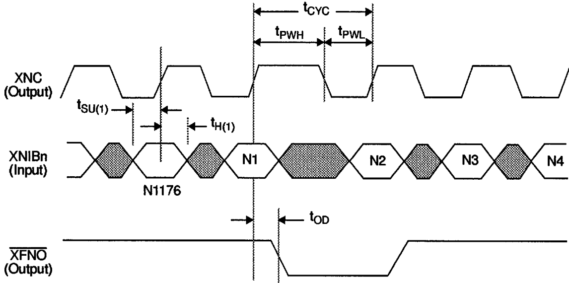
Figure 6. Terminal Side Transmit Nibble Input Timing
