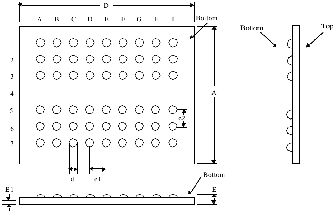
Figure 4: Center-Bonded WBGA Package
