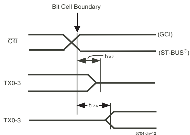
Figure 9. Serial Outputs and External Control
