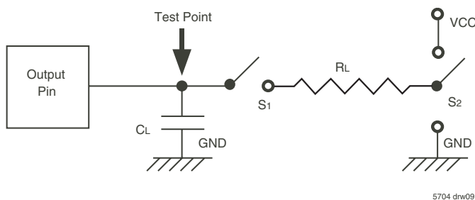
Figure 6. Output Load
