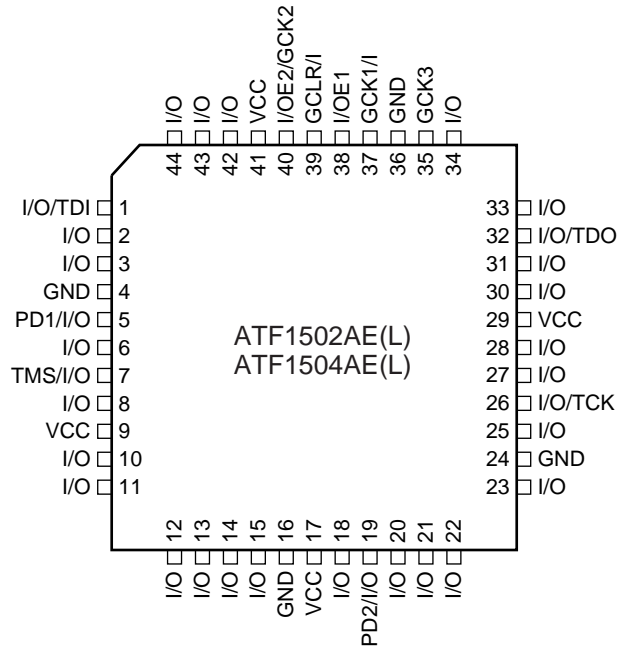
44-lead TQFP
