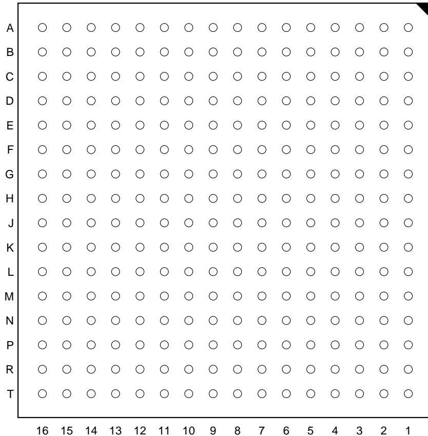
256-ball 1.0 mm Pitch – Bottom View
