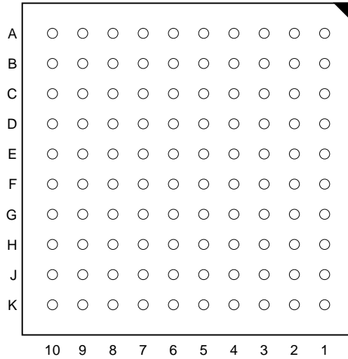
100-ball 1.0 mm Pitch – Bottom View
