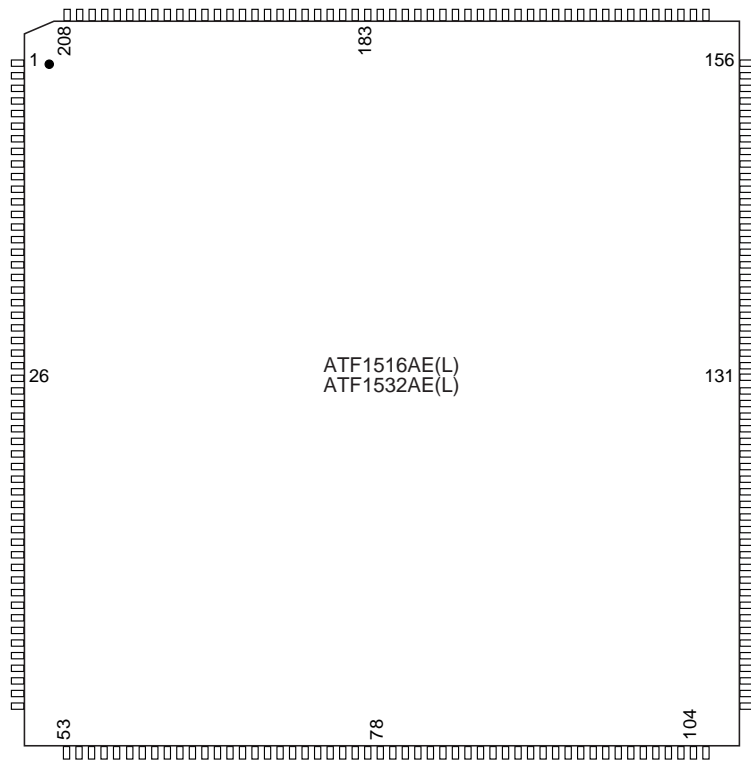
208-lead PQFP – Top View
