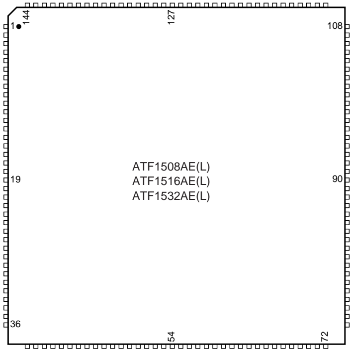
144-lead LQFP – Top View
