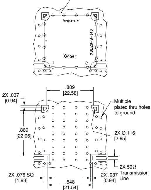
Dimensions are in Inches [Millimeters] XDL20-8-140 Mounting Footprint
