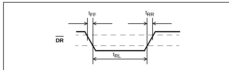
Figure 8 - \overline{DR} Output Timing
