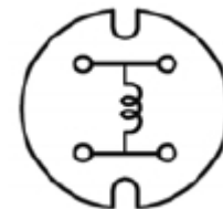
CIRCUIT FOR VALUES FROM 18□H ~ 1000□H
