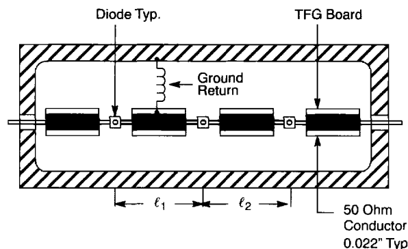
Figure 5. Top View
