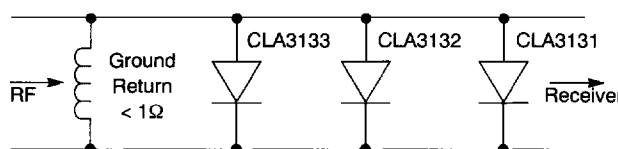
Figure 1. Cascaded Limiter Design
