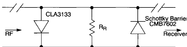
Figure 2. Quasi-Active Limiter
