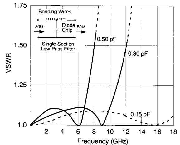
Figure 8. Typical VSWR for Low Pass Filters
