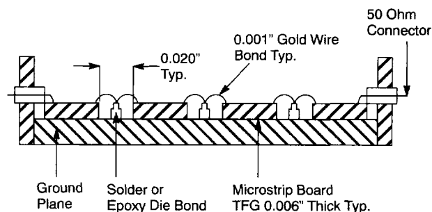
Figure 4. Side View
