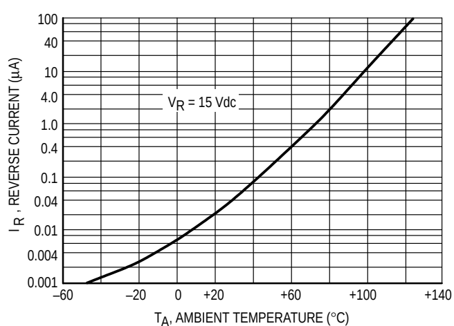
Figure 4. Leakage Current
