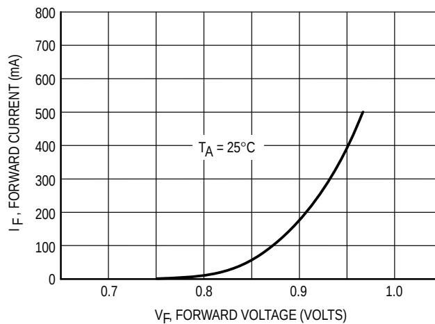
Figure 2. Forward Voltage
