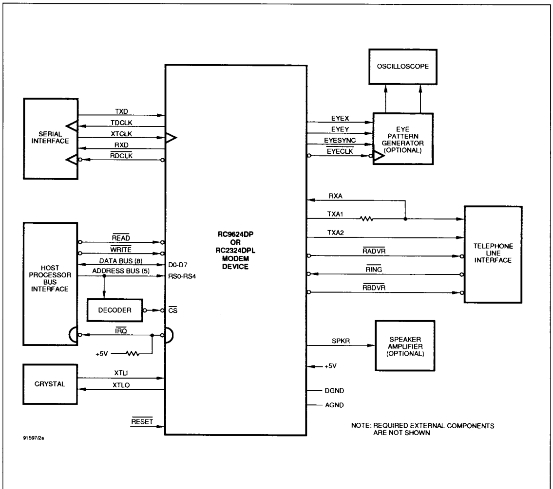
Figure 2. RC9624DP Functional Interface Signals
