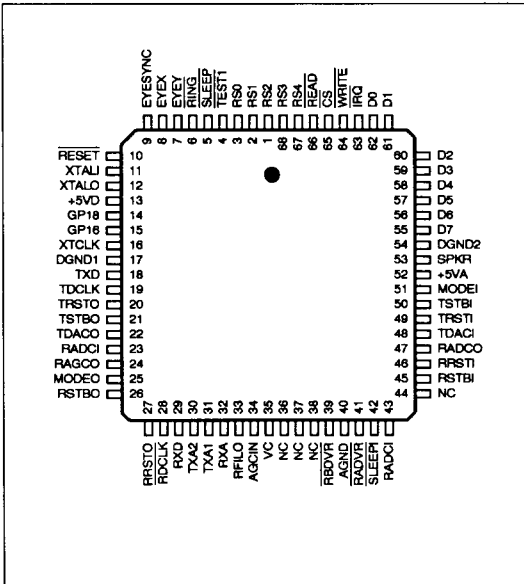
Figure 3. RC9624DP Pin Signals
