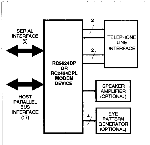
Figure 1. RC9624DP OR RC2424DPL Modem General
