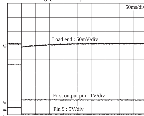
Falling (V9 ⇒ low) characteristics
