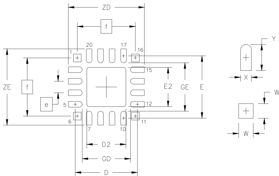
Figure 19. PCB Land Pattern
