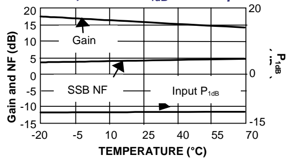
Gain, NF and P 1dB vs. Temperature
