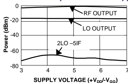
Power Output vs. Power Supply
