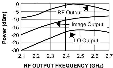
Power Output vs. RF Frequency
