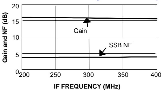
Gain and Noise Figure vs. IF Frequency
