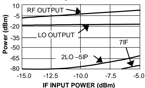
Power Output vs. IF Power
