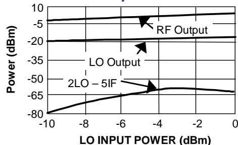
Power Output vs. LO Power
