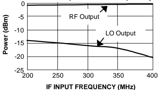
Power Output vs. IF Frequency
