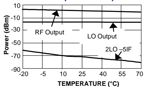
Power Output vs. Temperature
