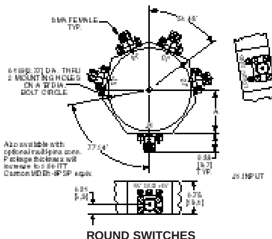
ROUND SWITCHES
