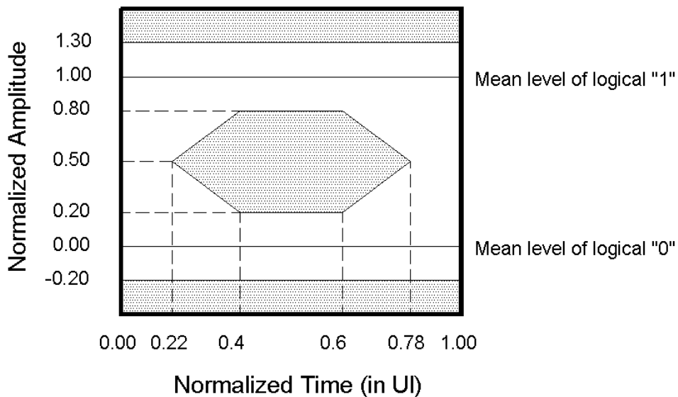
Transmitter eye Diagram mask
