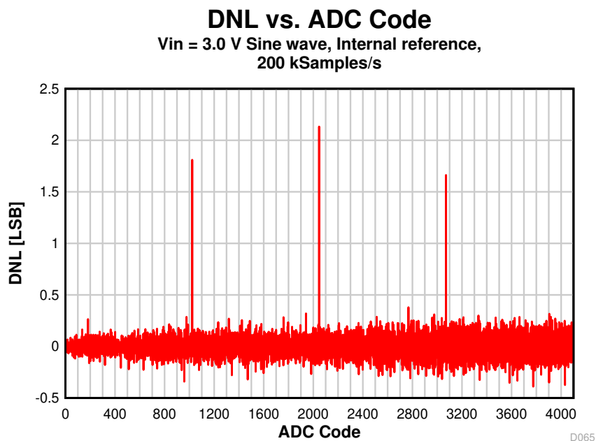
Figure 8-23. DNL vs. ADC Code
