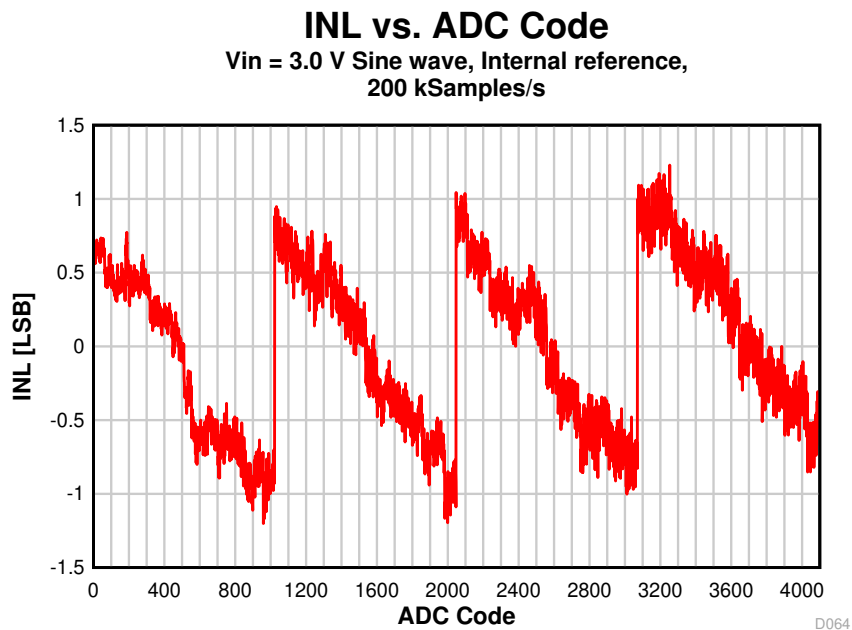
Figure 8-22. INL vs. ADC Code
