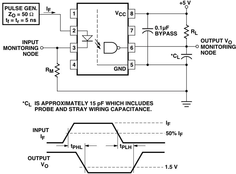
Figure 7. Test Circuit for t_{PHL} and t_{PLH} .
