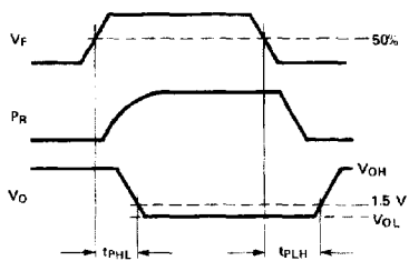
Figure 26. Propagation Delay Test Waveforms.
