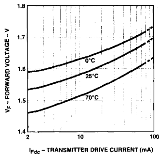
Figure 9. Typical Forward Voltage vs. Drive Current.
