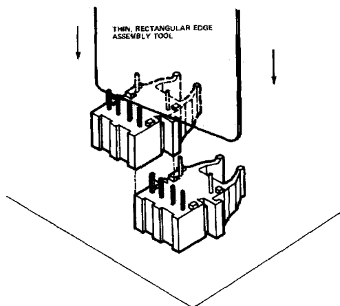
Figure 1. Interlocked (Stacked) Horizontal or Vertical Packages.
