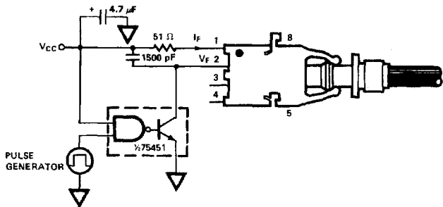
Figure 16. 1 Mbd Propagation Delay Test Circuit.
