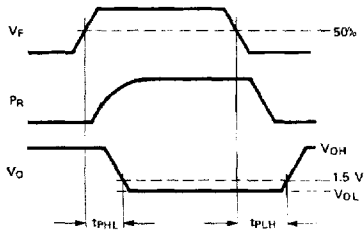
Figure 19. Propagation Delay Test Waveforms.
