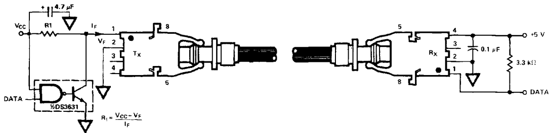
Figure 20. Typical 40 kBd Interface Circuit.
